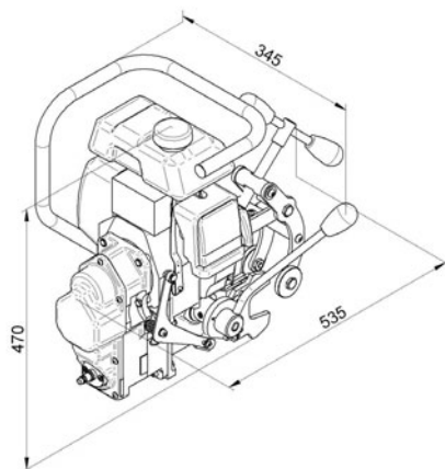
RailMAB 960
