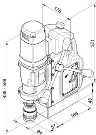
MAB 455
