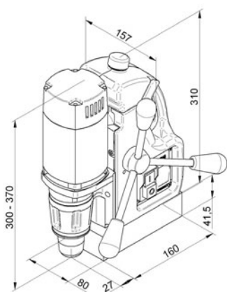
MAB 455
